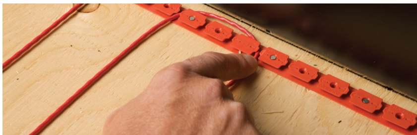
FIGURE 2.26 : Installer le câble chauffant
