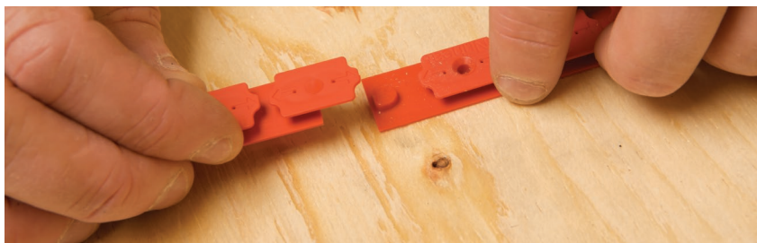
FIGURE 2.25: Snap together Nuheat Cable Guides
